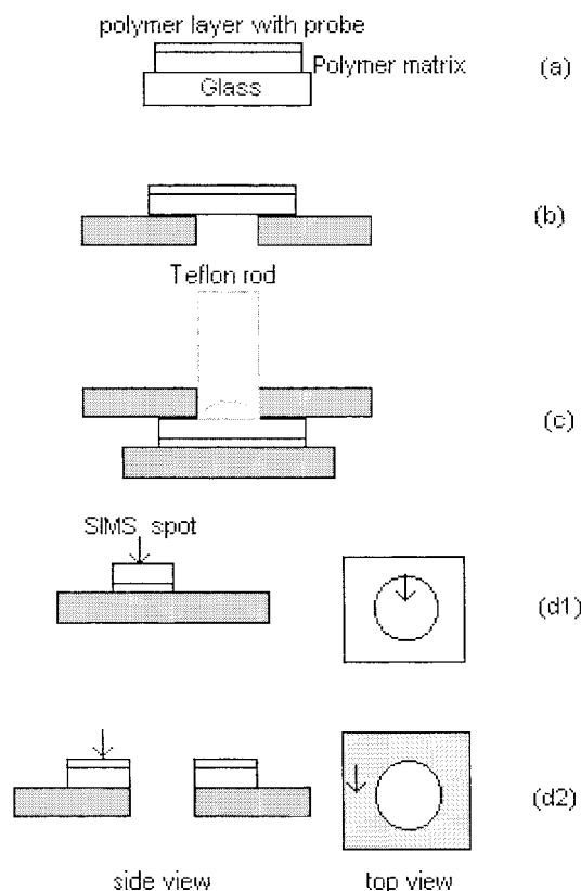
Figure 1. Schematic of the process for making free-standing films and transferring them onto substrates for DSIMS measurements. (a) A bilayer film is first floated onto a glass slide. (b) The bilayer is then floated onto a silicon substrate with a 4 mm hole where it is annealed. (c) After annealing the free-standing portion is transferred by pressing with a Teflon rod onto a Si wafer for DSIMS analysis. (d) Two sample geometries for the DSIMS analysis and location of the DSIMS sputtering beam: (1) transferred portion of the free-standing film; (2) supported section of the film, adjacent to the hole in the Si wafer.
